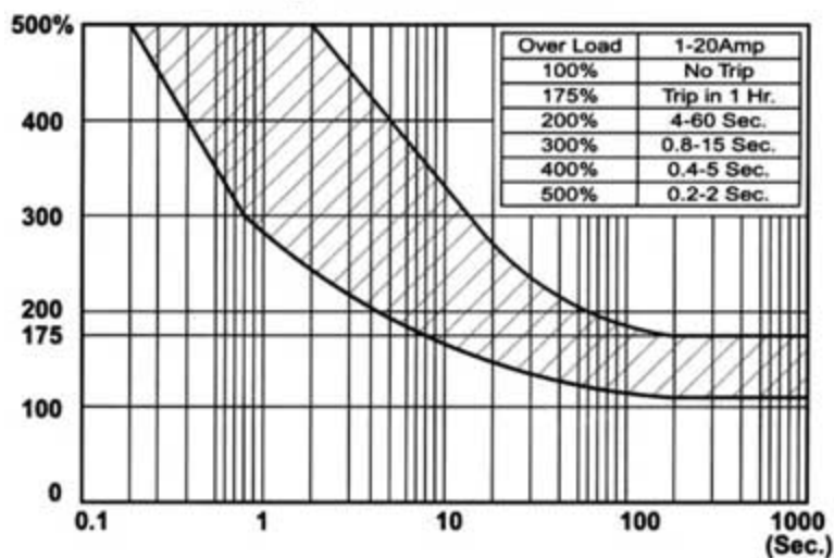
Trip Time Curves
