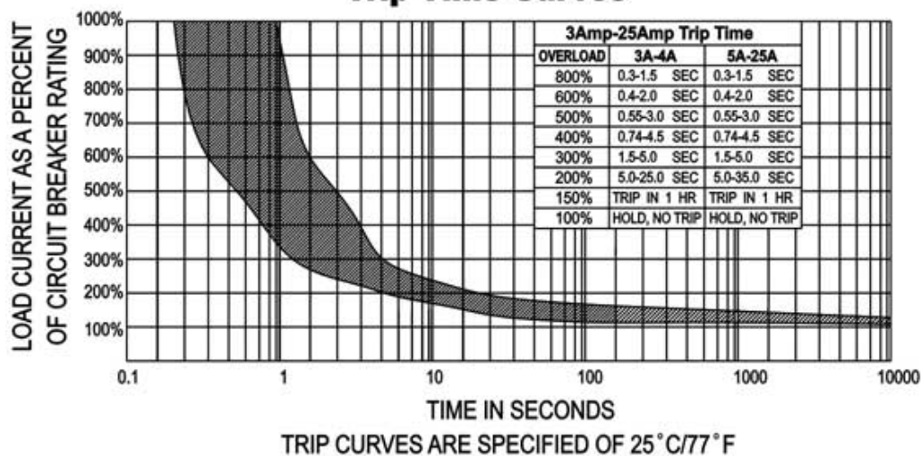
Trip Time Curves
